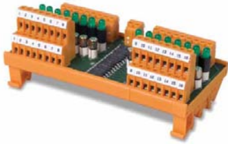
Custom Interface: LED and Fuse Module
